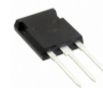
APT50GT120B2RDQ2G Microsemi Corporation IGBT 1200V 94A 625W TO247
