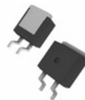
IXSA10N60B2D1 IXYS IGBT 600V 20A 100W TO263
