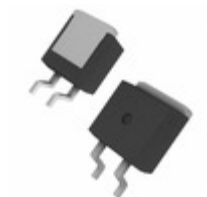
IXSA15N120B IXYS IGBT 1200V 30A 150W TO263AA
