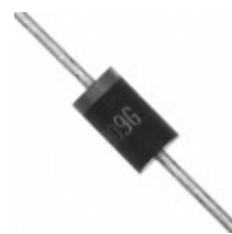
UF5403-E3/73 Vishay Semiconductor Diodes Division DIODE GEN PURP 300V 3A DO201AD
