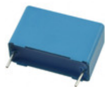
B32523Q1685K189 EPCOS (TDK) CAP FILM 6.8UF 10% 100VDC RADIAL
