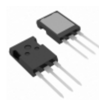
IXGX32N170H1 IXYS IGBT 1700V 75A 350W PLUS247
