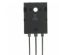
APT50GT120LRDQ2G Microsemi Corporation IGBT 1200V 106A 694W TO264
