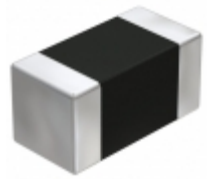
UMK105CG331JVHF Taiyo Yuden CAP CER 330PF 50V NP0 0402
