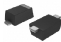
PMEG2005EH,115 Nexperia DIODE SCHOTTKY 20V 500MA SOD123F
