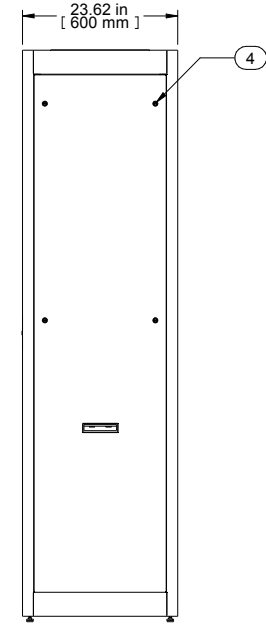
R.S. VIEW
