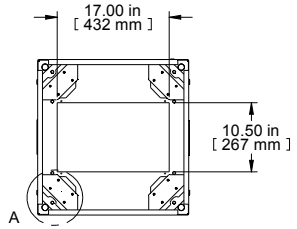
BOTTOM VIEW BOTTOM OPENING
